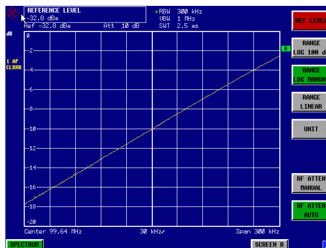
Fig. 2.20 Filter edge of a 300 kHz filter used as an FM-discriminator characteristic
